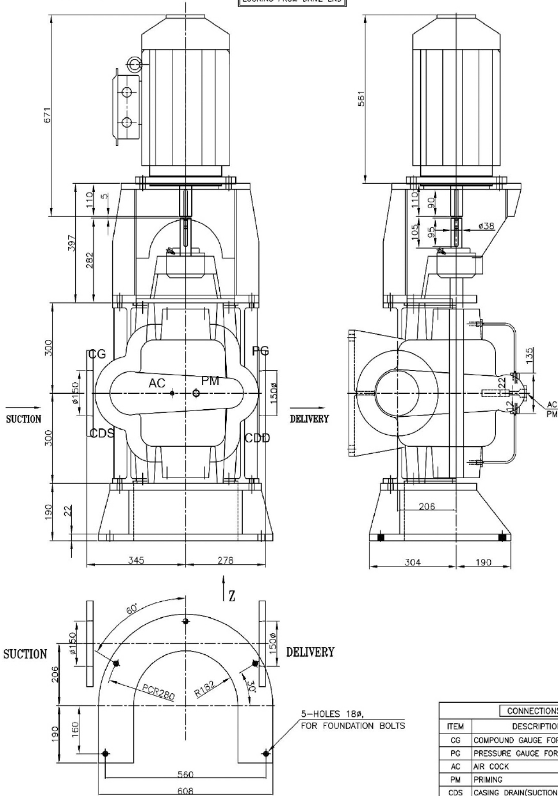
PLAN VIEW DIRECTION -Z (PUMP STOOL FEET DETAILS)
