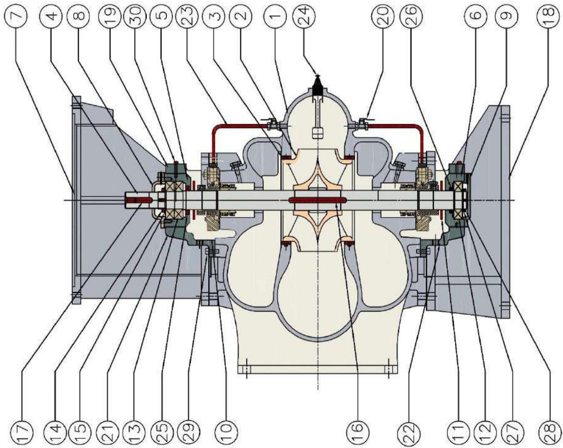
CROSS SECTIONAL DRAWING FOR SINGLE STAGE VERTICAL SPLIT-CASE PUMP WITH EXTERNAL BOTTOM BEARING AND CATRIDGE MECHANICAL SEALS
