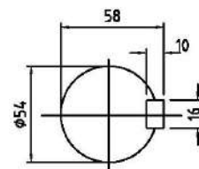
SCALE - 5:1 DETAIL OF SHAFT AT COUPLING END
