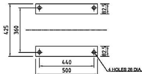
PLAN OF PUMP FEET
