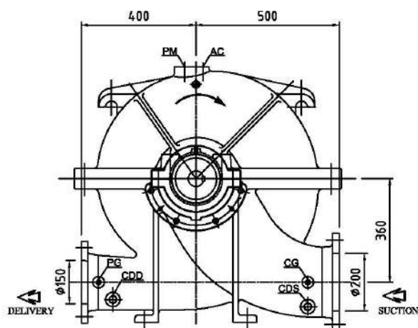
VIEW IN DIRECTION OF 'Z'
