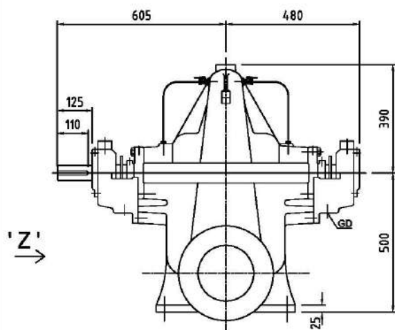
GENERAL ARRANGEMENT DRAWING FOR SINGLE STAGE AXIALLY SPLIT CASE PUMP MODEL - 6HS23
