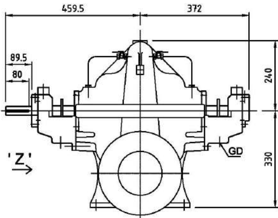
GENERAL ARRANGEMENT DRAWING FOR SINGLE STAGE AXIALLY SPLIT CASE PUMP MODEL - 5HS13
