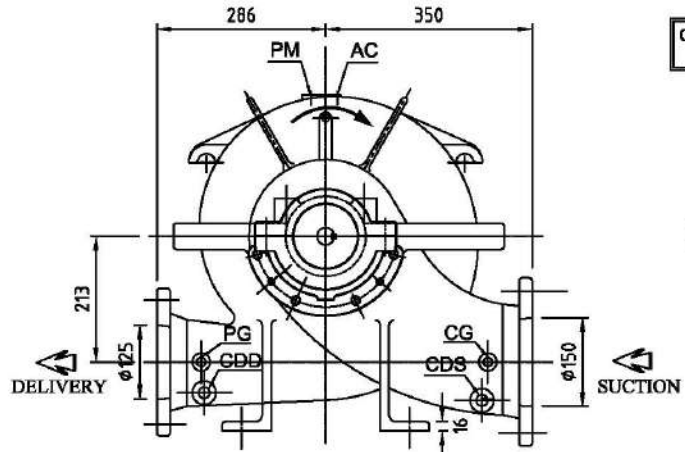
GENERAL ARRANGEMENT DRAWING FOR SINGLE STAGE AXIALLY SPLIT CASE PUMP MODEL - 5HS13
