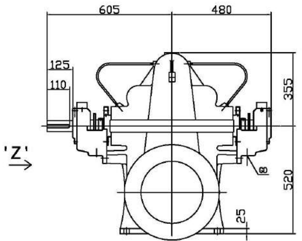
GENERAL ARRANGEMENT DRAWING FOR SINGLE STAGE AXIALLY SPLIT CASE PUMP MODEL – 10HS15L
