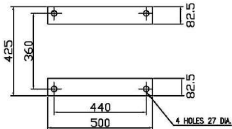
PLAN OF PUMP FEET
