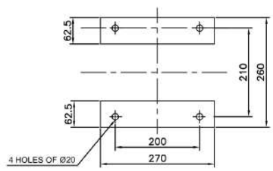
PLAN OF PUMP FEET
