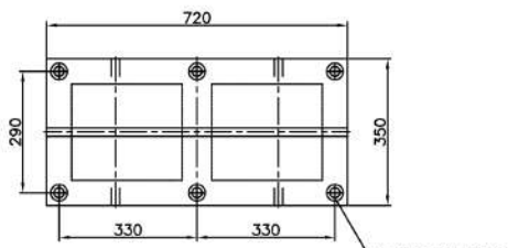
PLAN OF PUMP FEET
